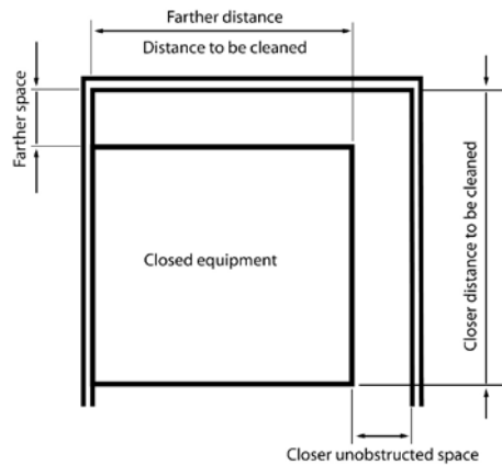
Figure 8d - Unobstructed direct cleaning space, cleaning behind a corner
